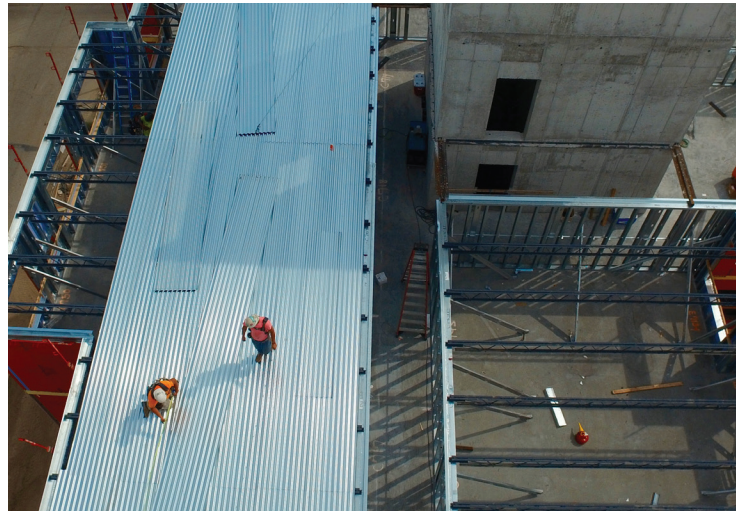
Ecospan is installed quickly and easily, with the decking providing a safe surface for construction crews without the need for shoring. Photo courtesy Rick Gilchrist Co., Inc.
